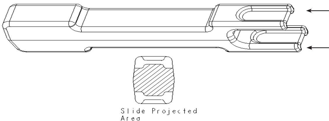
Fig. 4A-1A PROPOSED COMPONENT WITH ADDED FEATURES AND DESIGN MODIFIED FOR COST-EFFECTIVE DIE CASTING PRODUCTION, SHOWING ORIENTATION IN THE DIE CASTING DIE AND CORE SLIDE (MOVING DIE COMPONENT) TO CAST THE ADDITIONAL FEATURES.
